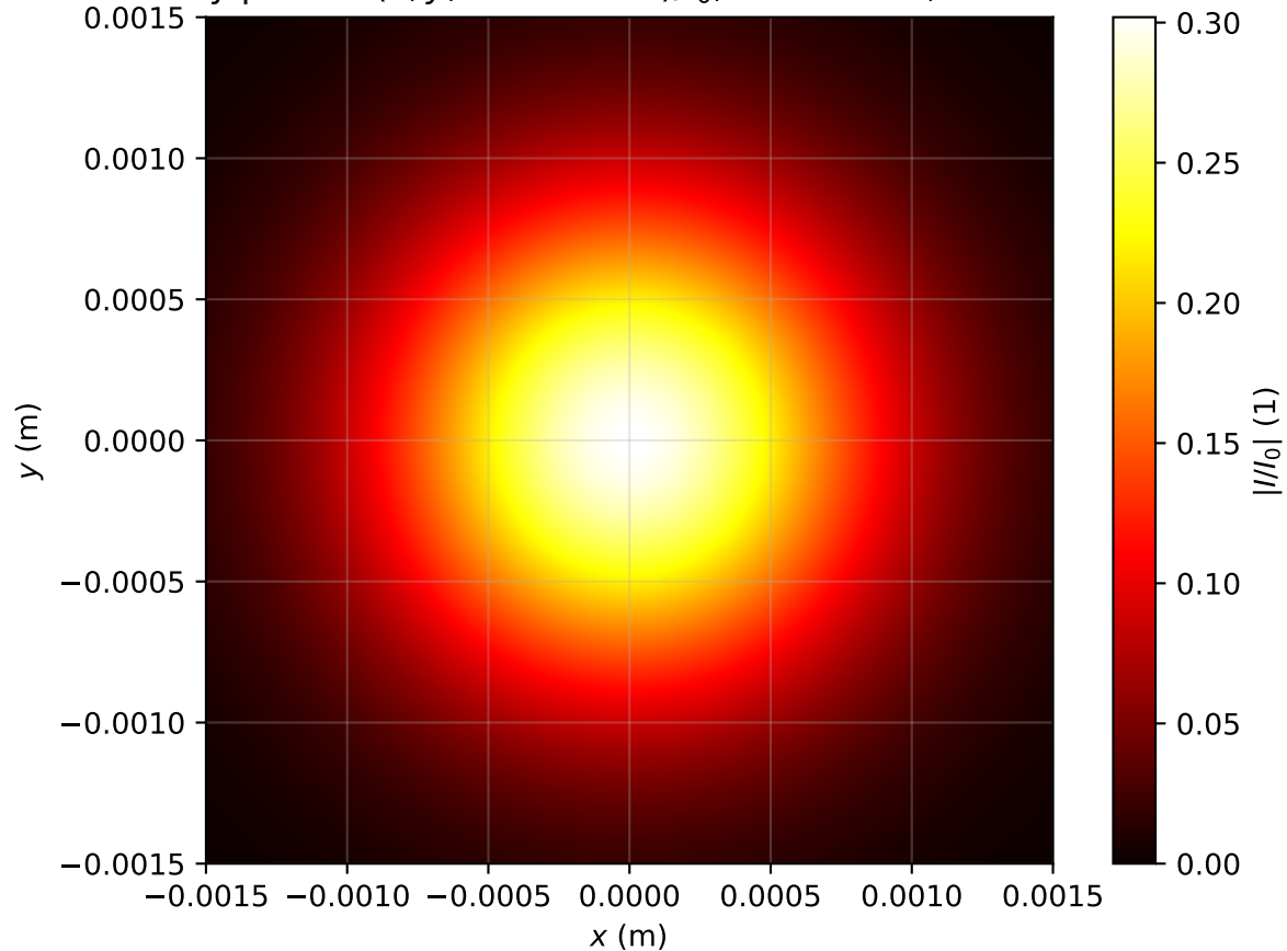
Intensity profile I(x, y, z = 3.503m)/I_0 , P_{in}=0.2P_{cr} , artificial time
